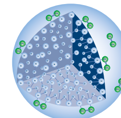
Competitive Phase Partially hybrid phase
