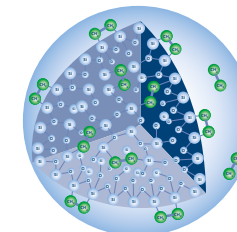
ASTRA® C-18 Hybrid Fully hybrid phase
